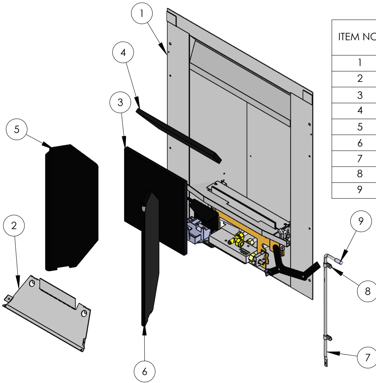
Slimline 3 Main Assembly
